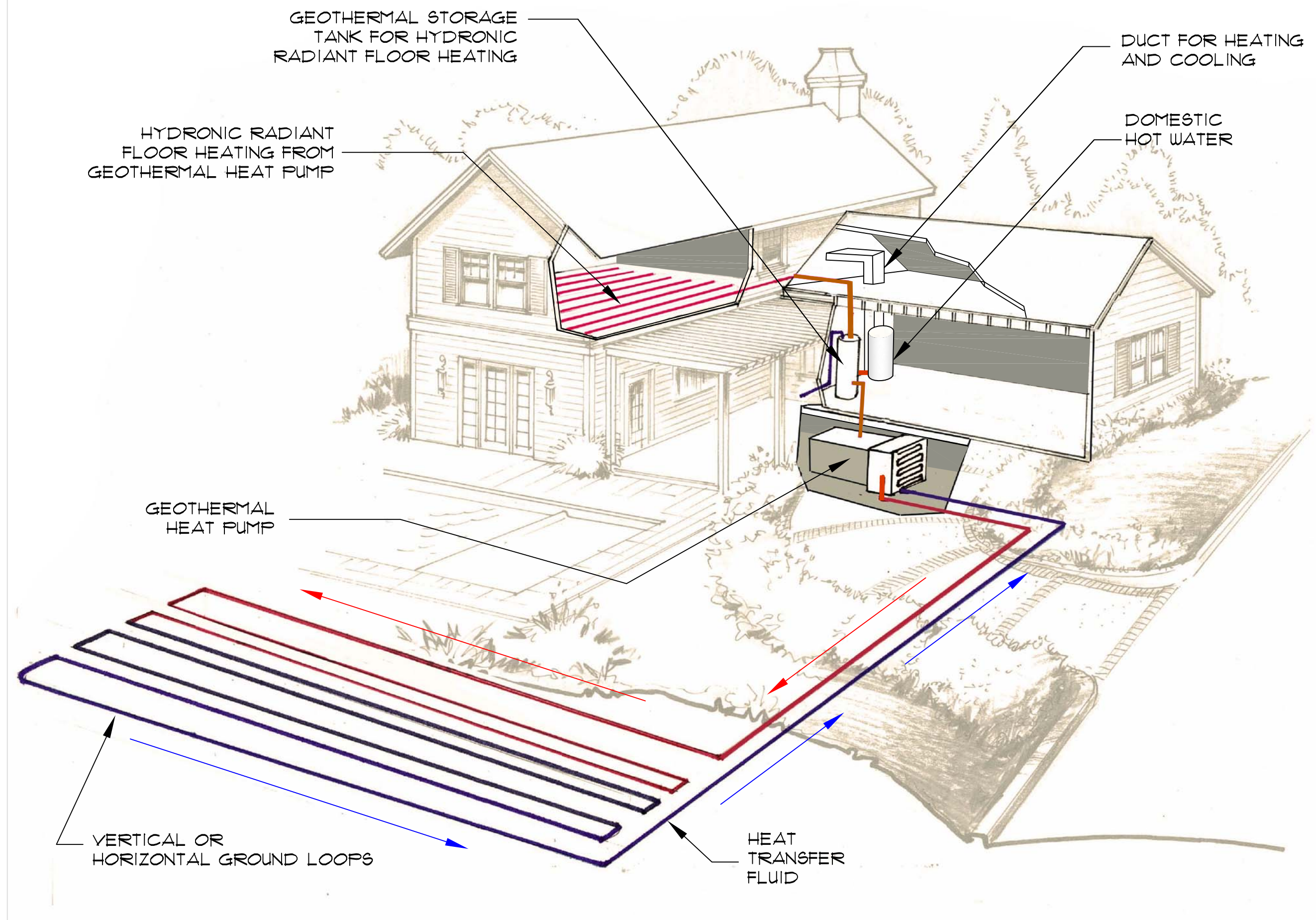
GEOTHERMAL AIR CONDITIONING SYSTEM
